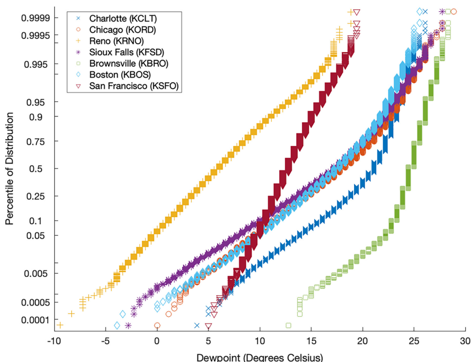
FIGURE 1 Cumulative distribution of daily-maximum T_d during June–September 1948–2020 for seven representative stations [Colour figure can be viewed at wileyonlinelibrary.com ]
